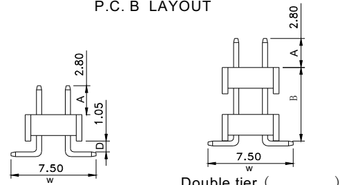
Double tier ( )
